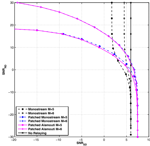
Fig. 8. Comparison of the Monostream and Alamouti relaying scheme for different activation time of the relay in DDF and Patched DDF protocols for M = 5, 6 . N_r = 2 , m_S = 2 , T_1 = K/m_S , and T_1/T_{i,i \geq 1} = 3 , Target outage probability of 10^{-2} .
