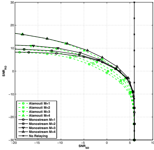
Fig. 7. Comparison of the Monostream and Alamouti relaying scheme for different activation time of the relay in DDF protocols for M = (1, 2, 3, 4) . N_r = 2 , m_S = 2 , T_1 = K/m_S , and T_1/T_{i,i \geq 1} = 3 , Target outage probability of 10^{-2}
