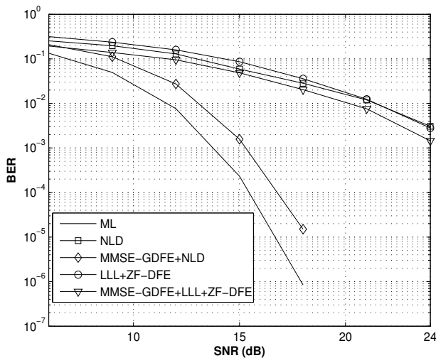
Fig. 4. Bit Error Rate vs. SNR for the Perfect Code 4 \times 4 using 16-QAM constellations.
