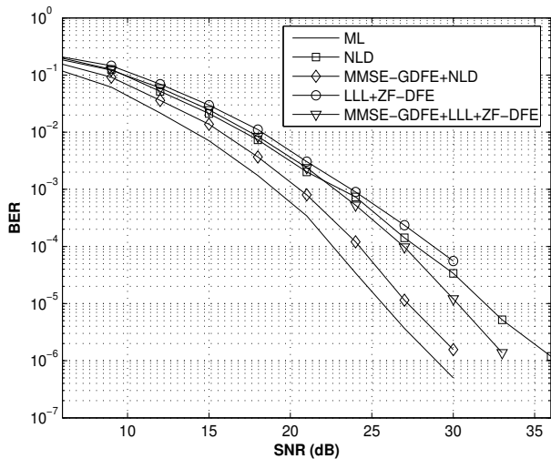
Fig. 3. Bit Error Rate vs. SNR for the Golden Code using 16-QAM constellations.
